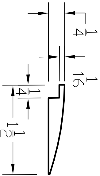
\frac{1}{4} " Reducer
