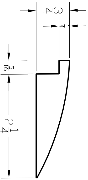
\frac{3}{4} " Reducer
