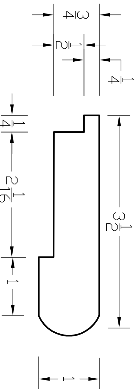
\frac{3}{4} " Stairnose
