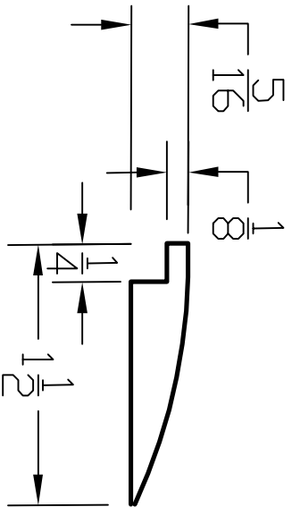
\frac{5}{16} " Reducer
