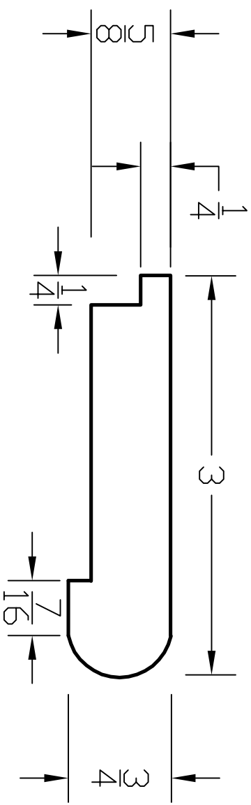
5/8" Stairnose
